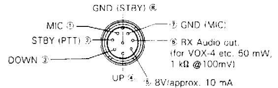
MIC connector (Front view)
